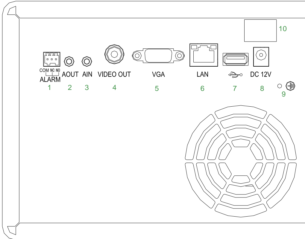
Rear panel of the VSR0804S
